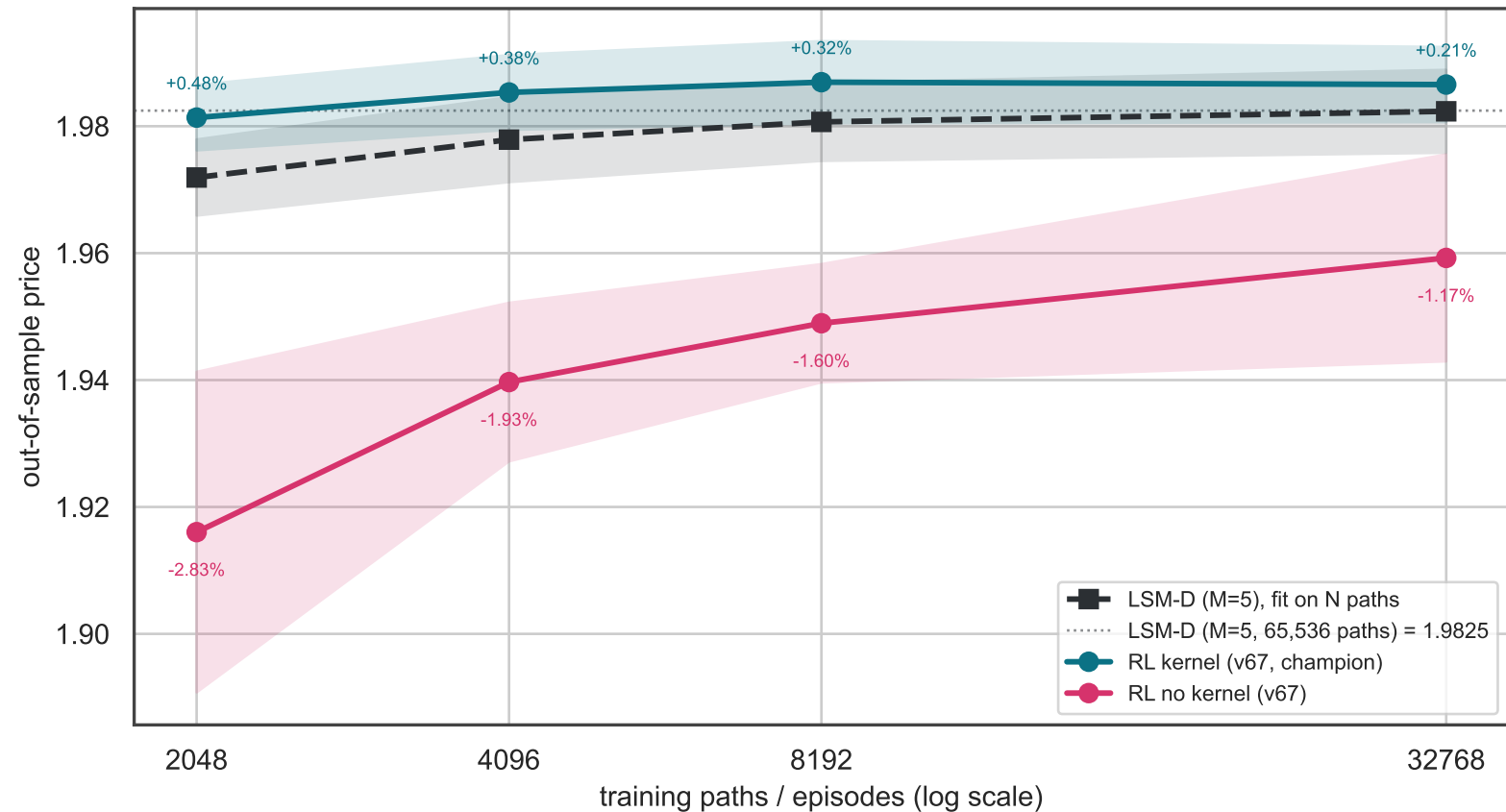
R2 · Sample efficiency — v67 kernel vs no kernel vs LSM-D (focal c=0.04 , \gamma=2 )
